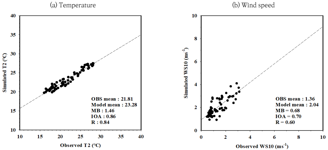
Fig. 6. Observed and simulated for (a) 2-m temperature and (b) 10-m wind speed during the study period.
